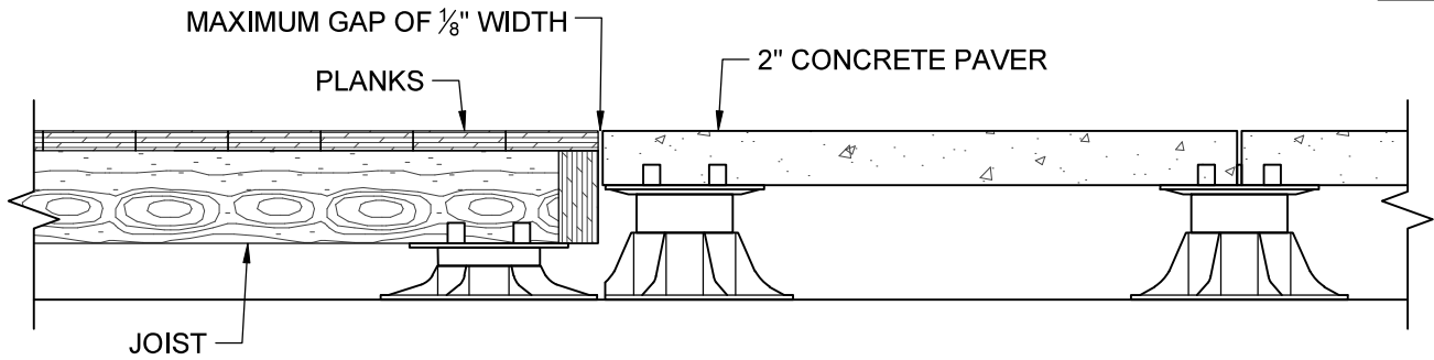
JOIST AND PLANK WITH 2" CONCRETE PAVER
