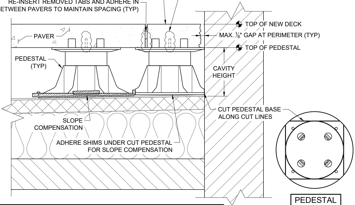
NARROW & SMALL CUT PAVER PERIMETER PLACEMENT
